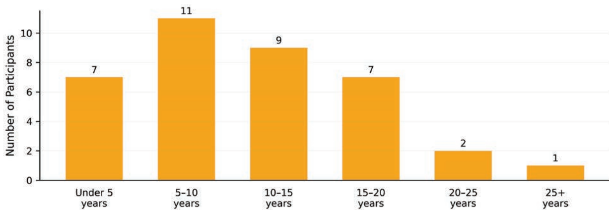
Figure 9. Sentence Length
